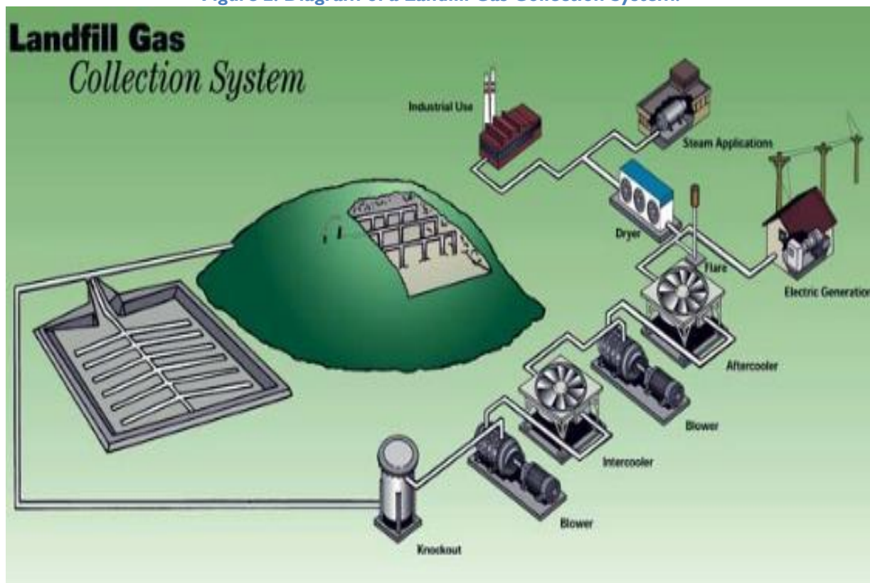
Figure 2: Diagram of a Landfill Gas Collection System.
