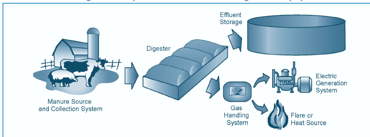
Figure 1: Components and Products of a Biogas Recovery System.
